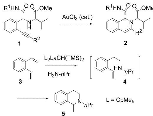
Figure 1. Published approaches to THIQs using hydroamination.
