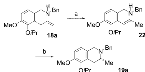
Scheme 3. Reagents and conditions: (a) n BuLi (2 × 16 mol-%), room temp., 18 h, 96%; (b) n BuLi (16 mol-%), 60 °C, 18 h, NMR spectra identical to that obtained in Scheme 1.
