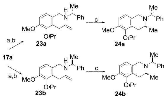
Scheme 4. Reagents and conditions: (a) ( R )- or ( S )-1-phenylethylamine, p -TSA, benzene or toluene, Dean–Stark apparatus, reflux, 18 h; (b) NaBH 4 , MeOH, H 2 O (1 drop), 0 °C to room temp., 18 h; (c) n BuLi (2 × 16 mol-%), room temp., 6 h, then 60 °C, 18 h. For yields see Table 3.
