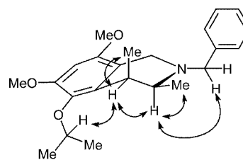
Figure 5. nOe interactions for the cis -isomer of 19c .
