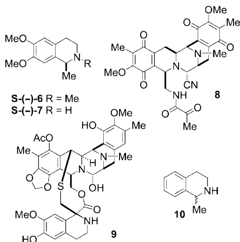
Figure 2. Topical examples of THIQs.
