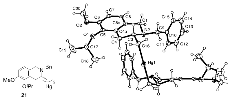
Figure 4. ORTEP diagram of the X-ray crystal structure of compound 21 (ellipsoids shown at 30% probability).
