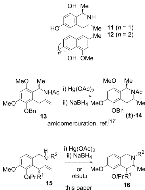
Figure 3. Our group's approaches to substituted THIQs.
